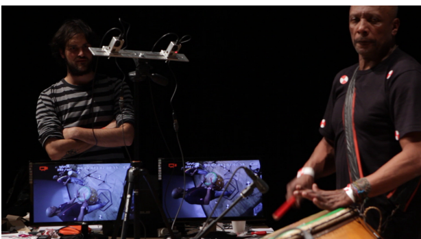
Figure 4. High-speed cameras in stereo pair with custom-made mounting, wired to two screens and power supply.
